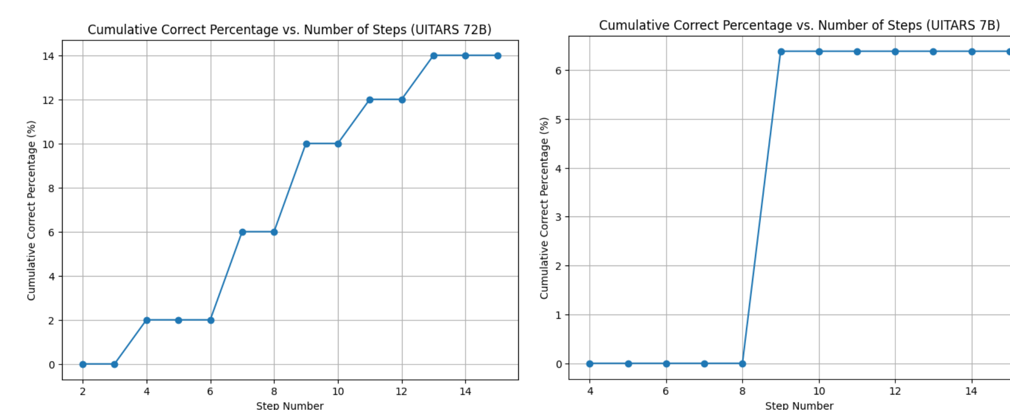
Fig. 7: UITARs 7B / 72B Scaling through 15 Steps (no MCTS)
