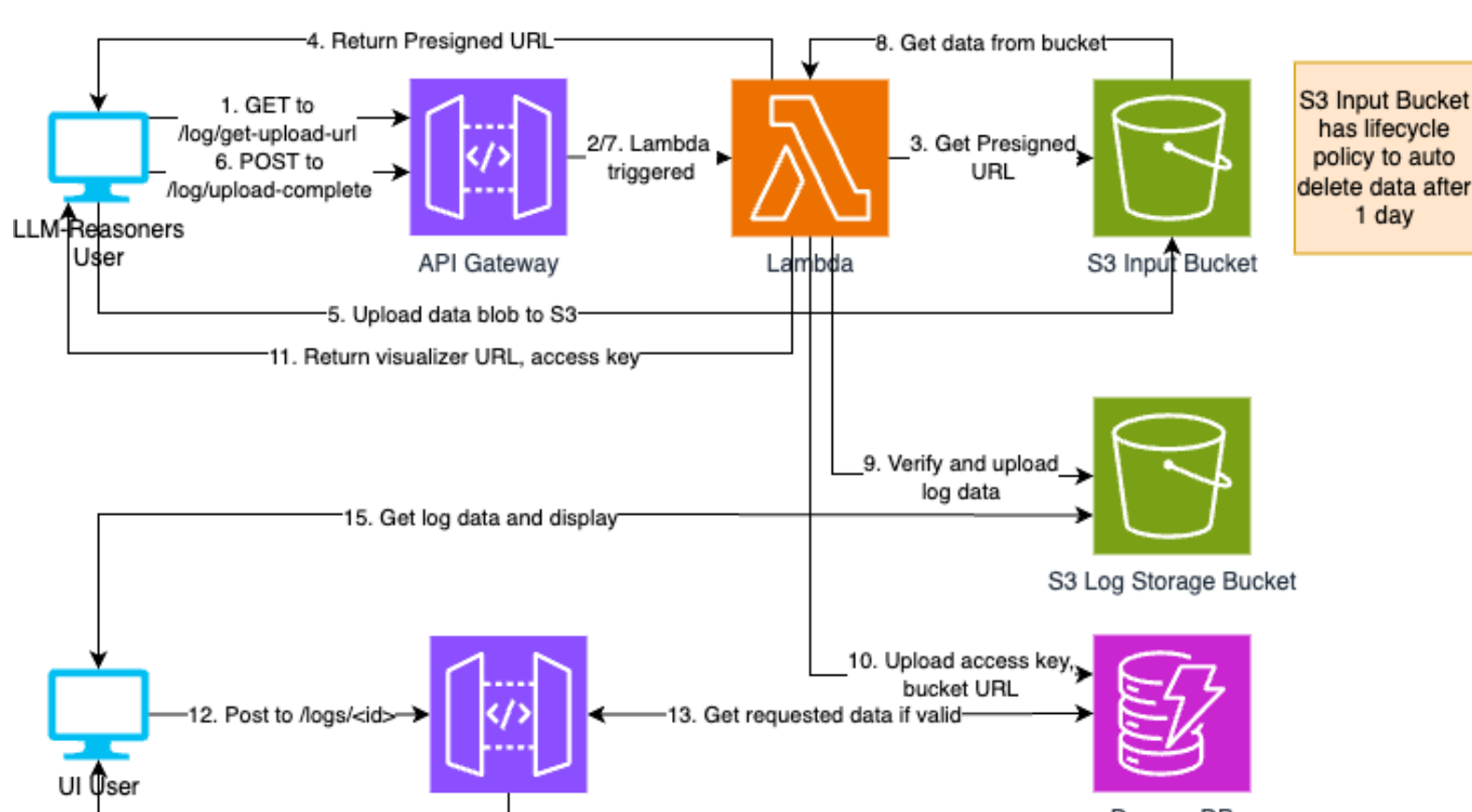
Fig. 2: Visualizer Architecture
