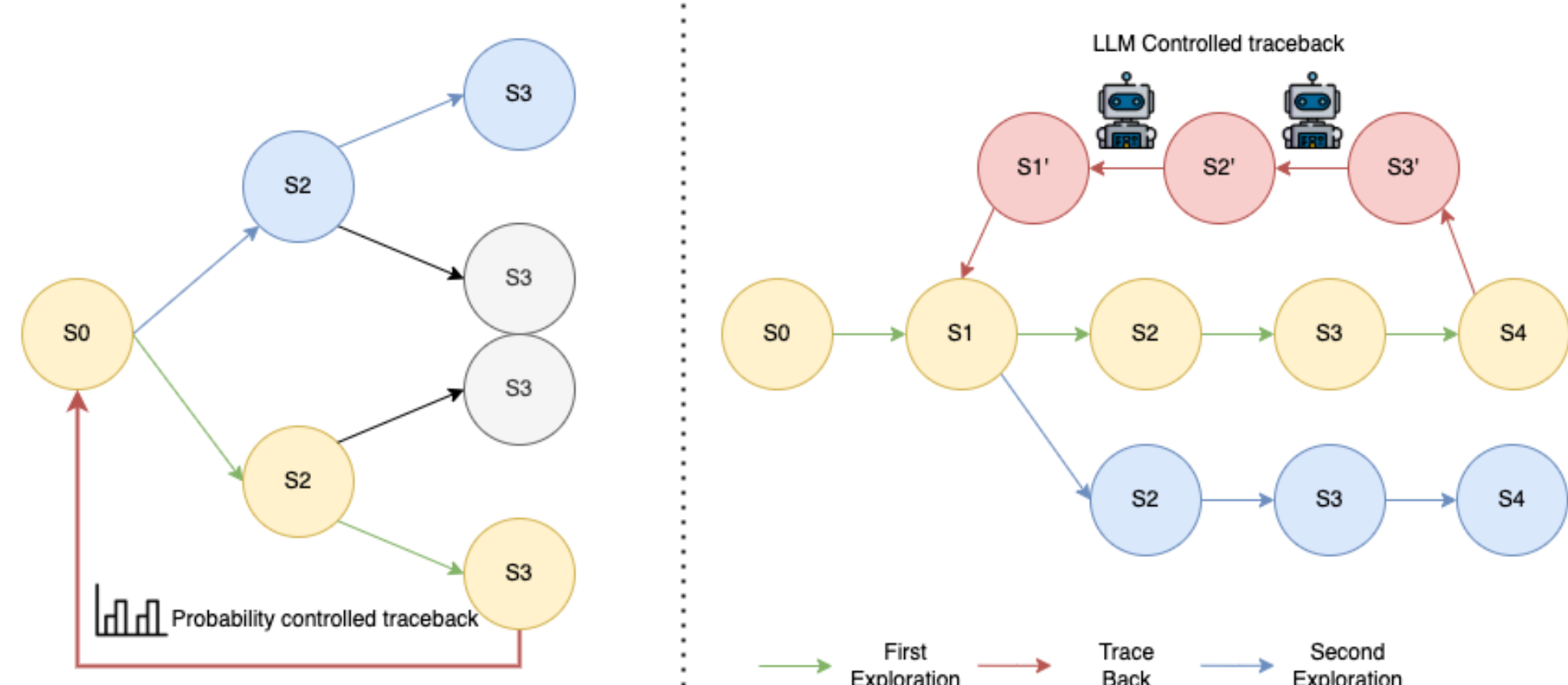
Fig. 3: Test-Time Scaling
